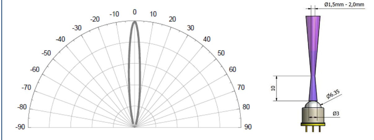
Angular Diagram / Beam Characteristics
