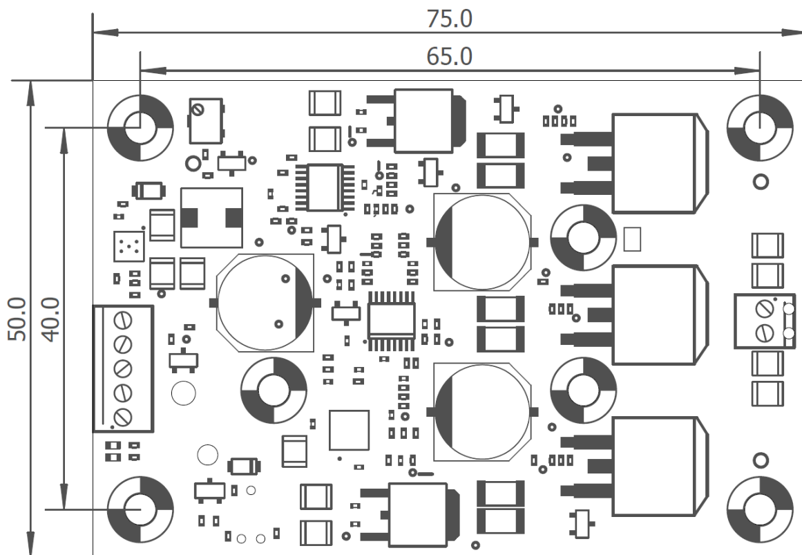
Fig. 12: PCB dimensions
