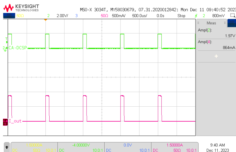
Fig. 9: Pulsed operation
