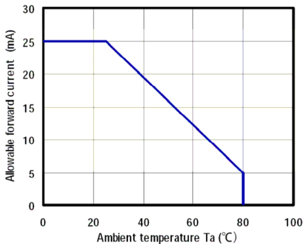
ambient temp.[°C] vs. max. forw. Current [mA]:
