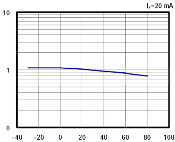
ambient temp.[°C] vs. max. forw. Current [mA]:
