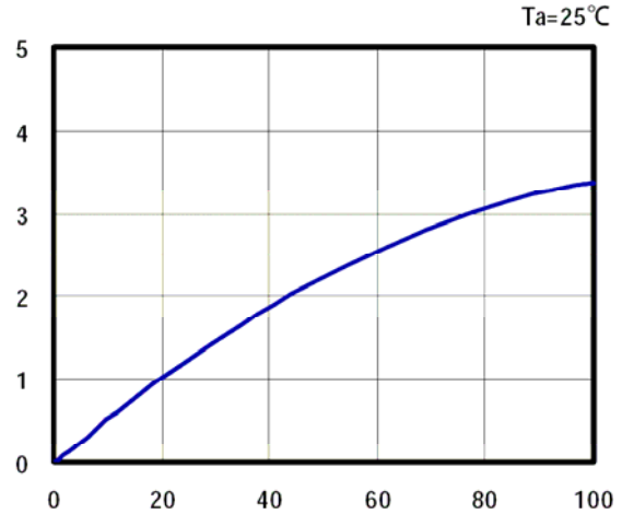
ambient temperature [°C] vs. forw. voltage [V]:
