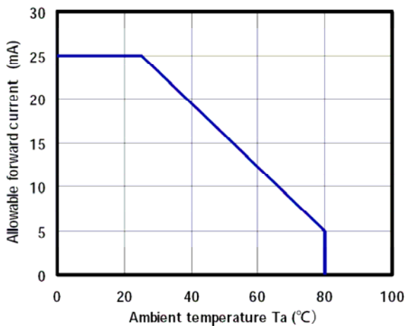
ambient temp. vs. maximum forward current:
