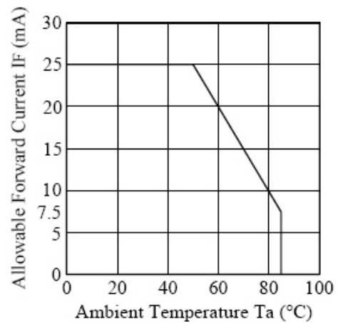
Ambient Temp. vs Allowable Forward Current:
