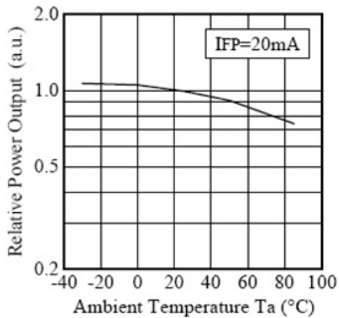
Ambient Temp. vs. Relative Output Power:
