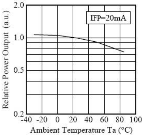
Ambient Temp. vs. Relative Output Power:
