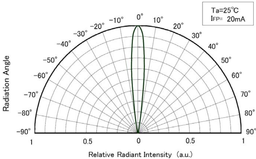
Directivity
